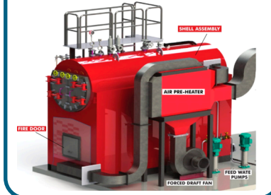
Multi Flame
